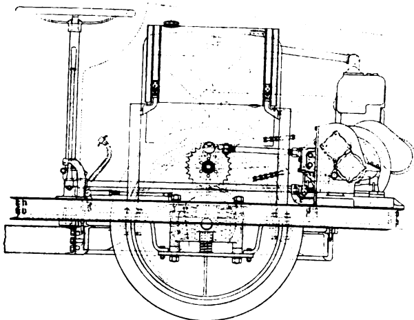
General layout of Truكتور power plant, transmission and steering mechanism
